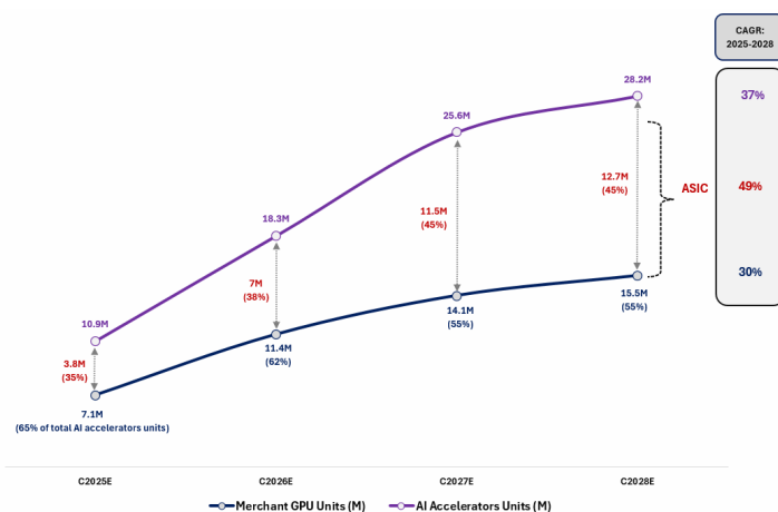
Figure 1. Accelerators GPU Trend
